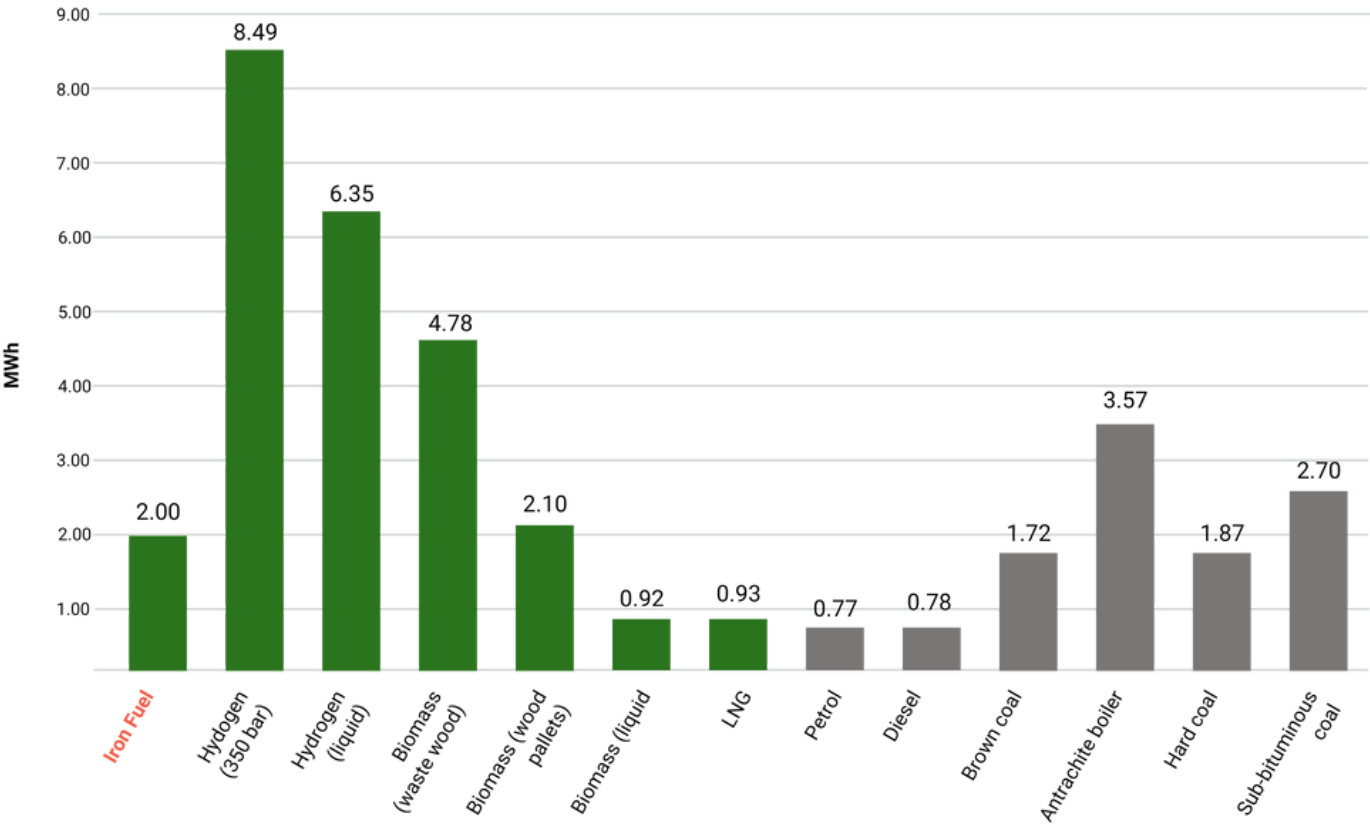
Transport Costs Comparison 100 km by truck
