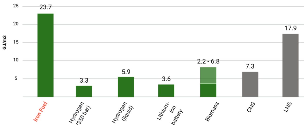
Thermic energy per volume A comparison with other alternatives
