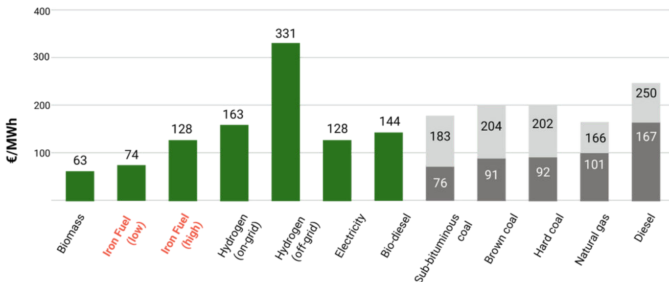
Cost of heat (current & incl. compensation costs) A comparison with other systems
